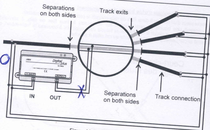
Figure 11: Wiring a turntable
